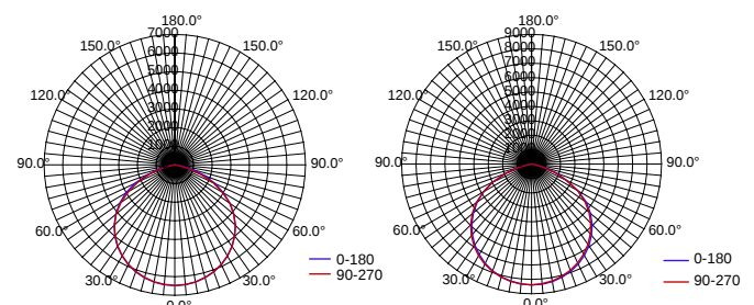
LF83R- 110W/19725lm
